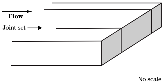
Figure 4-7 One joint set parallel to flow (resists erosion)
